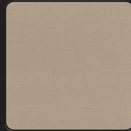
TOURMALINE
